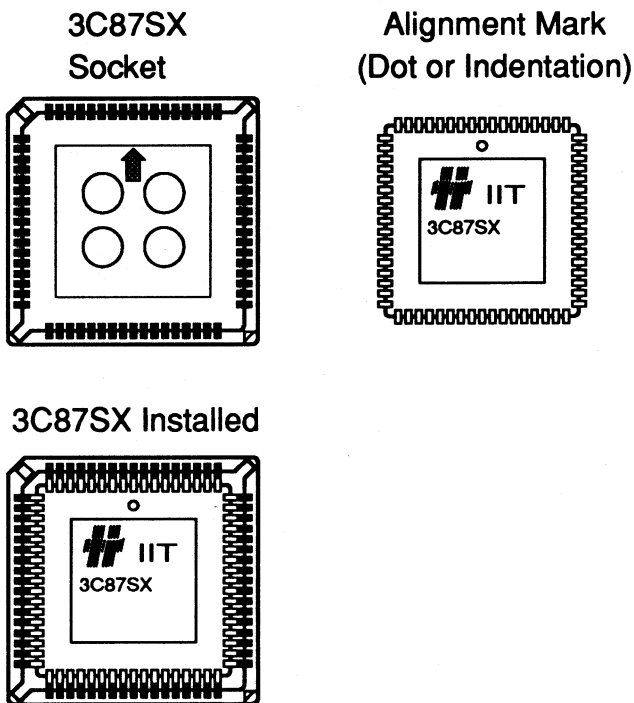
FIGURE 12 — TOP VIEW OF CHIP AND SOCKET
